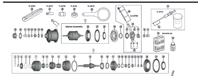
ALFINE 11-speed Internal Hub SG-S7001-11
